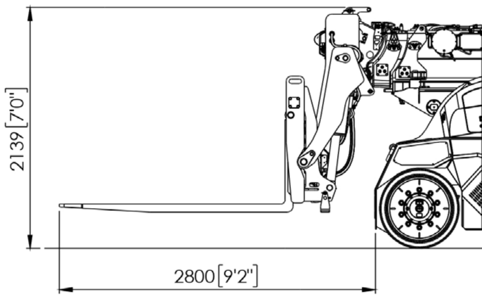
Fork on short boom
